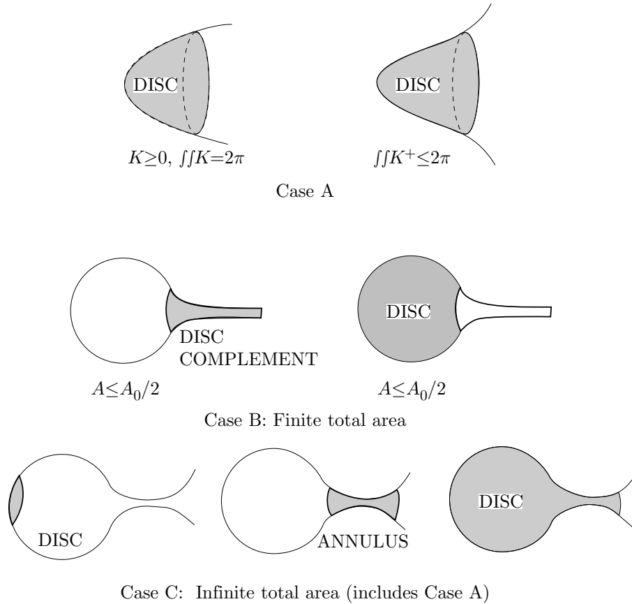
FIGURE 1. In a smooth, complete surface of revolution, with decreasing Gauss curvature K , a least-perimeter enclosure of prescribed area must consist of one or two circles about the origin, bounding a disc, the complement of a disc, or an annulus. (These surfaces cannot in general be isometrically embedded in \mathbf{R}^3 .)
