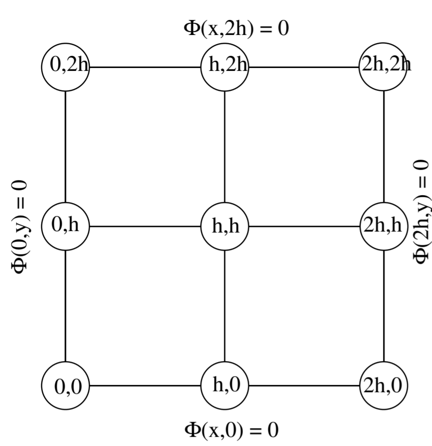
3 \times 3 grid for solution of the Poisson equation within a 2-dimensional square.
