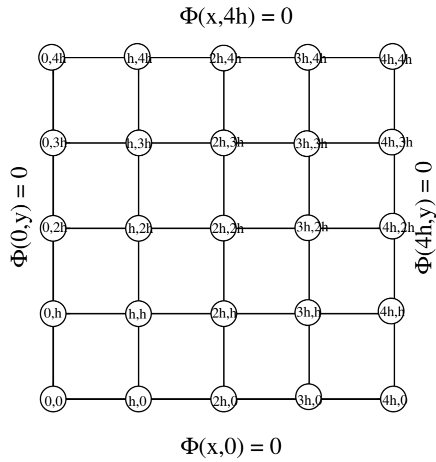
5 \times 5 grid for solution of the Poisson equation within a 2-dimensional square.
