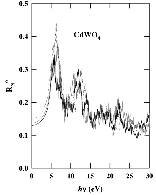
FIG. 12. Values of normal incidence reflectivity for \text{CdWO}_4 ; R_N^y (solid-black line), R_N^z (gray line) and R_N^x (dotted line), calculated from Eq. (5), neglecting off-diagonal dielectric contributions.
