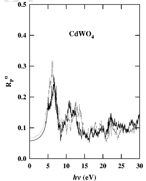
FIG. 13. Values of reflectivity for the z - x ( c - a ) face of \text{CdWO}_4 for p -polarization at incidence angle \theta=45^\circ ; R_p^z (solid black line) and R_p^x (dotted line), calculated from Eq. (8), neglecting off-diagonal dielectric contributions.
