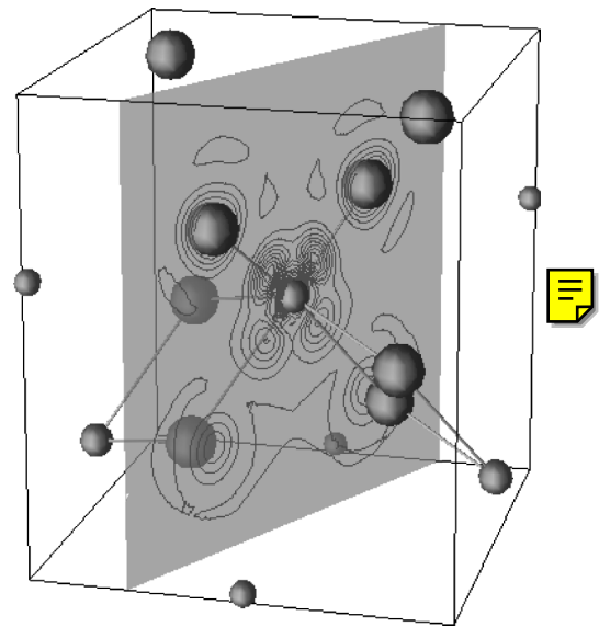
FIG. 5. A perspective drawing of the crystal structure of \text{CdWO}_4 . The spheres represent O, W, and Cd positions using large, medium, small sizes, respectively. The bonds represent the near-neighbor W-O interactions. The shaded plane is drawn to pass through a W atom and its nearest-neighbor O atoms. This is the plane that is used to construct the two-dimensional electron contour plots described below. The contours superimposed on this diagram correspond the upper-conduction-band states presented in Fig. 6(f).
