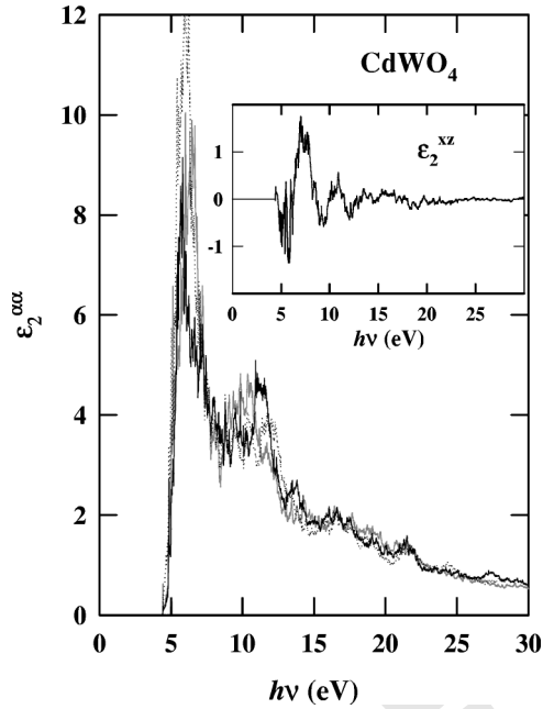
FIG. 10. Calculated values of \epsilon_2^{yy} (solid-black line), \epsilon_2^{zz} (dotted line), and \epsilon_2^{xx} (gray line) for CdWO 4 . Inset shows off-diagonal element \epsilon_2^{xz} .
