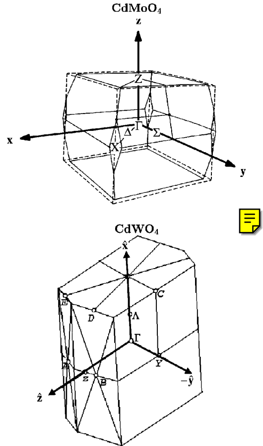
FIG. 3. Diagram of the Brillouin zones for \text{CdMoO}_4 and \text{CdWO}_4 .
