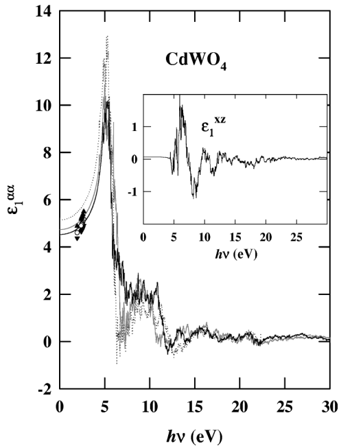
FIG. 11. Calculated values of \epsilon_1^{yy} (solid black line), \epsilon_1^{zz} (dotted line), and \epsilon_1^{xx} (grey line) for CdWO 4 . Experimental values from Ref. 29 are plotted with filled triangles and open circles corresponding to the three eigenvalues of \epsilon_1^{\alpha\beta} in the transparent region. Inset shows off-diagonal element \epsilon_1^{xz} .
