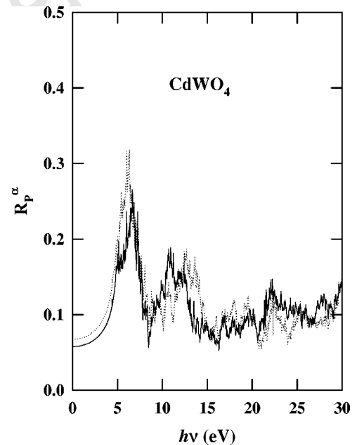
FIG. 13. Values of reflectivity for the z - x ( c - a ) face of CdWO 4 for p -polarization at incidence angle \theta=45^\circ ; R_p^z (solid black line) and R_p^y (dotted line), calculated from Eq. (8), neglecting off-diagonal dielectric contributions.
