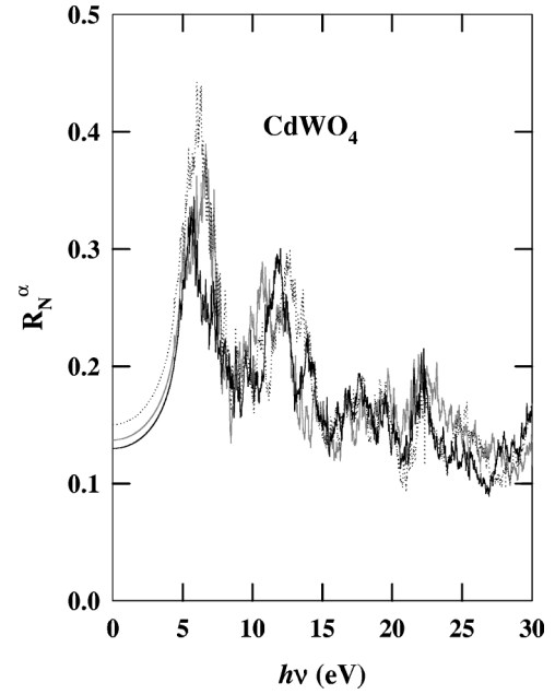
FIG. 12. Values of normal incidence reflectivity for CdWO 4 ; R_N^y (solid-black line), R_N^z (gray line) and R_N^x (dotted line), calculated from Eq. (5), neglecting off-diagonal dielectric contributions.
