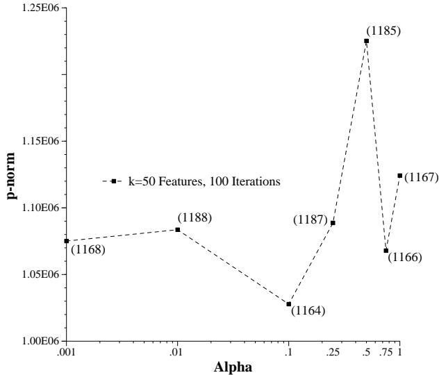
Fig. 1. Reduction in \|\mathbf{W}\|_p / \|\mathbf{W}\|_1 ( p -norm) for p = 0.5 as the smoothing parameter \alpha is increased for the nonnegative matrix factorization \mathbf{A} = \mathbf{W}\mathbf{H} of the Enron noun-by-message matrix. Elapsed CPU times (seconds) for CNMF to produce k = 50 features in 100 iterations are provided in parentheses.
