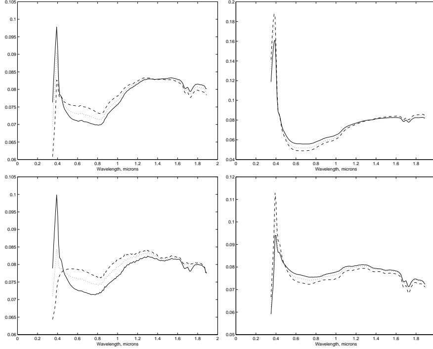
Fig. 4. Representative simulated spectral traces from \mathbf{Y}_i ( i = 1 : 4 ), where i is the dominant material in the mixture. (top-left) \mathbf{Y}_1 : Aluminum. (top-right) \mathbf{Y}_2 : Mylar. (bottom-left) \mathbf{Y}_3 Solar cell. (bottom-right) \mathbf{Y}_4 White paint.
