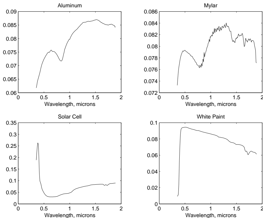
Fig. 3. Laboratory spectral signatures for aluminum, mylar, solar cell, and white paint. For details see (Luu et al., 2003).
