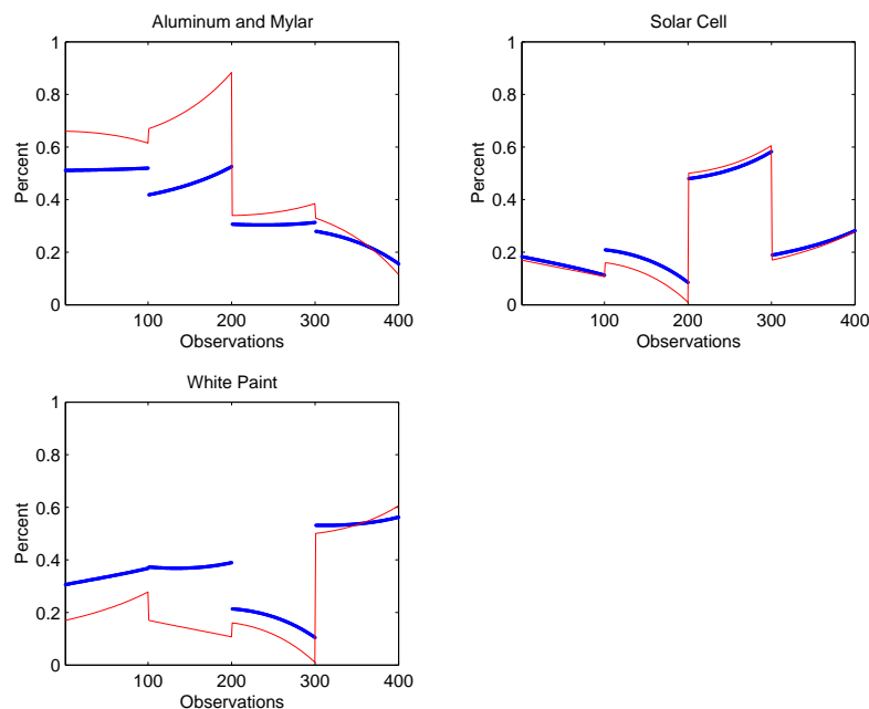
Fig. 6. Fractional abundances obtained using PMRNSD with \mathbf{B} \approx \mathbf{U} given in Figure 5. True fractional abundances are represented in red. The result of the approximation using PMRNSD is in blue.
